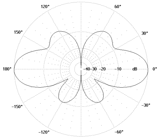
Vertical radiation diagram f = 156.8\text{MHz}
